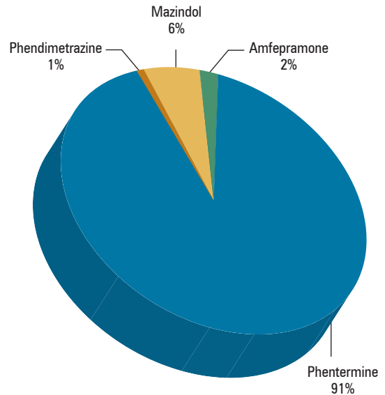
Figure 11. Central nervous system stimulants in Schedule IV: share of total reported manufacture, selected substances, 2015
